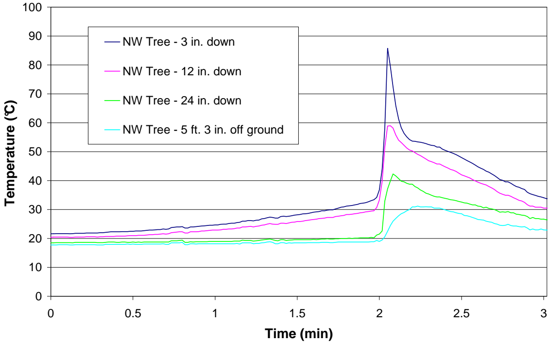
Figure 65 – Test 14 NW Tree
