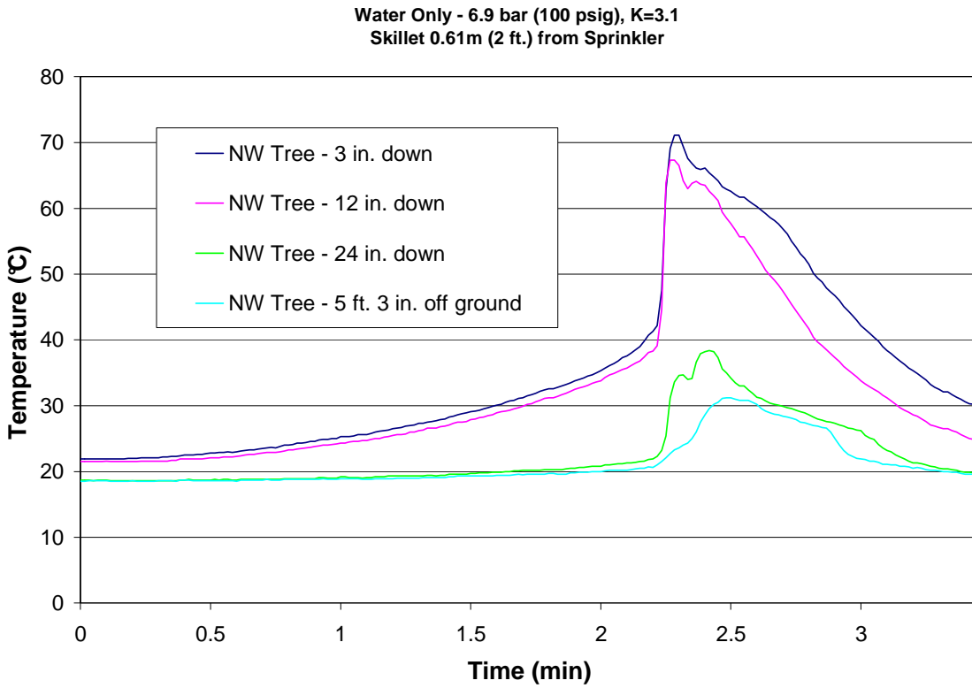
Figure 35 – Test 9 NW Tree
