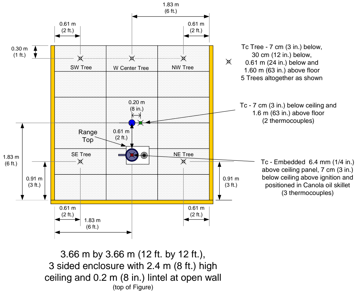
Figure 5 – Enclosure Testing Plan View (Tests 6 through 13)
