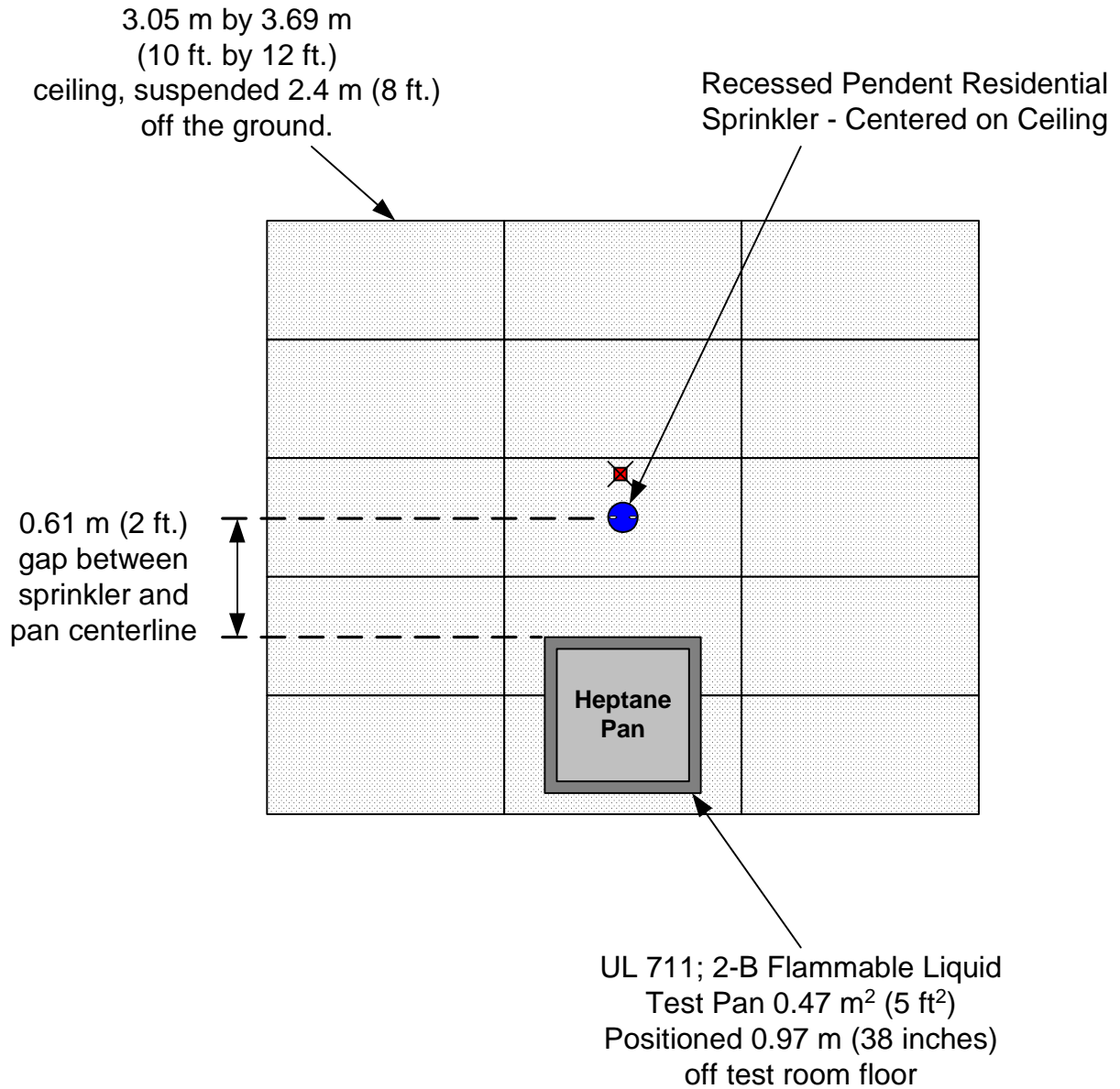
Figure 2 – Open Area Plan View (Tests 1 – 4, 16 and 17)
