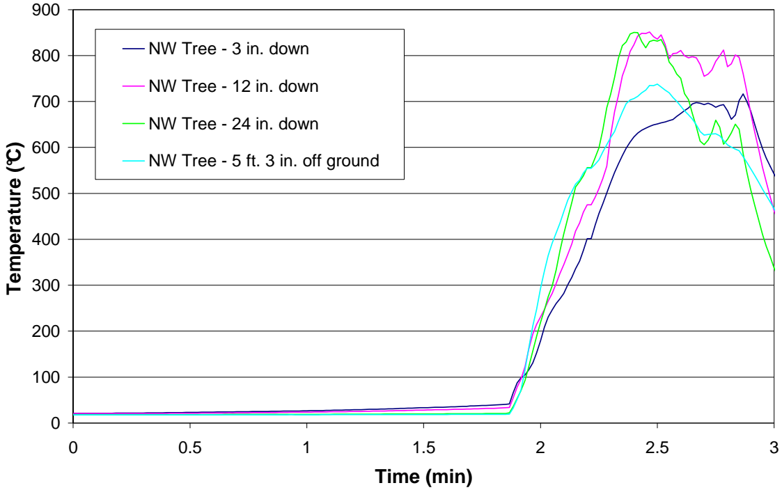
Figure 17 – Test 6 NW Tree
