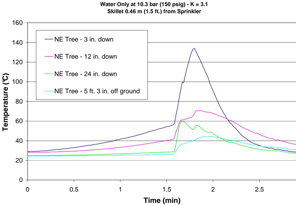
Figure 72 – Test 15 NE Tree
