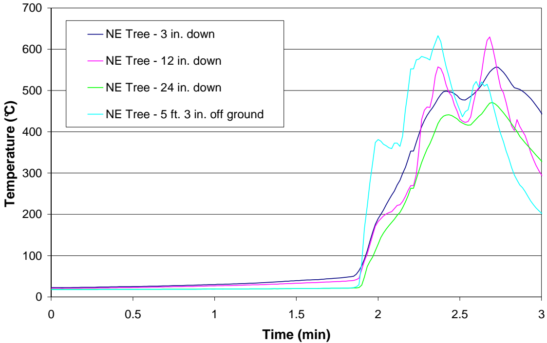
Figure 18 – Test 6 NE Tree
