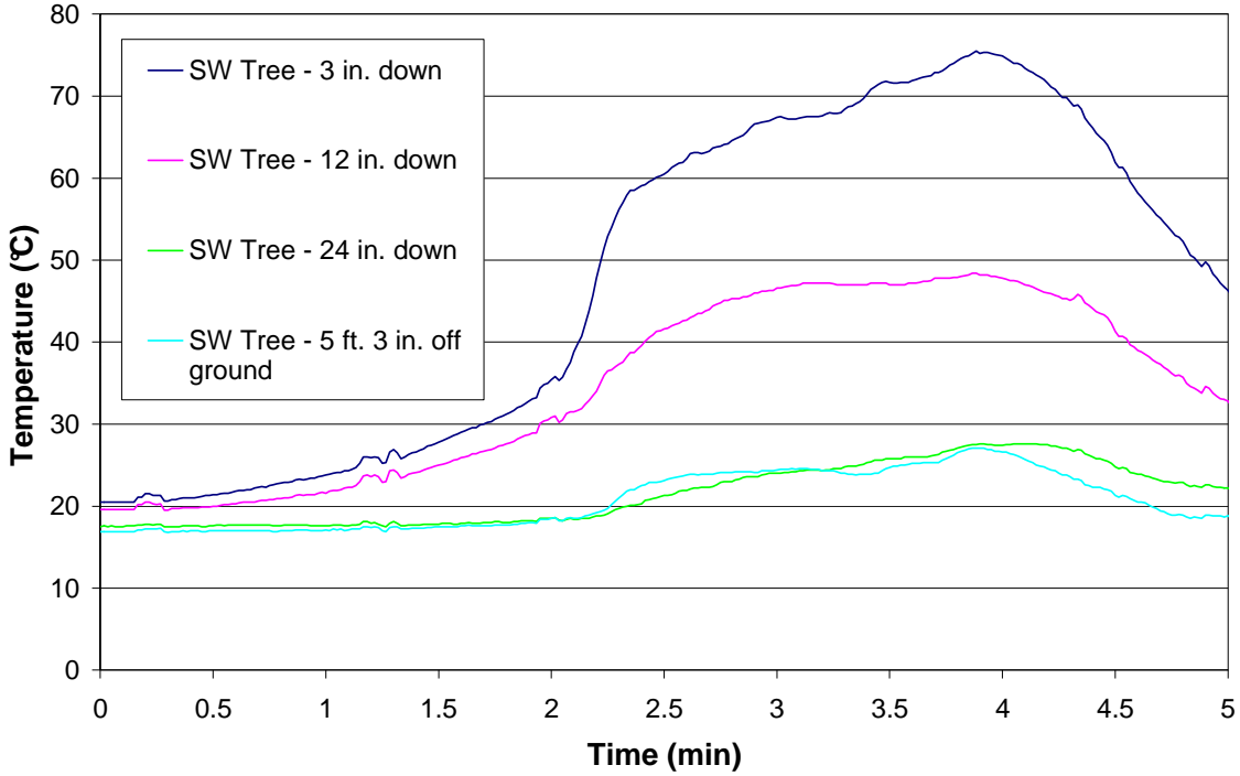
Figure 57 – Test 13 SW Tree
