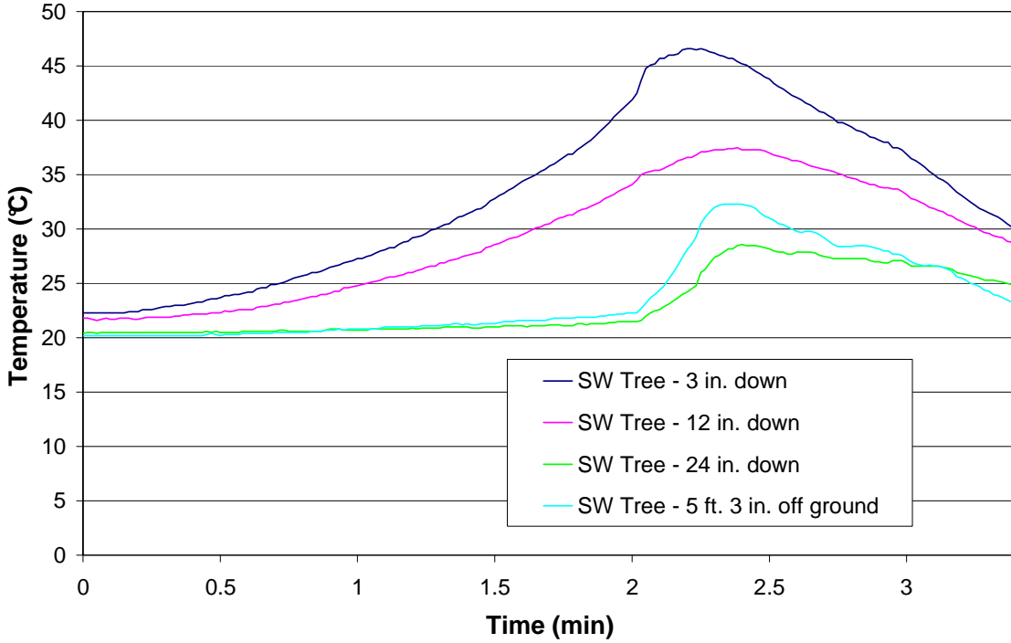
Figure 45 – Test 11 SW Tree
