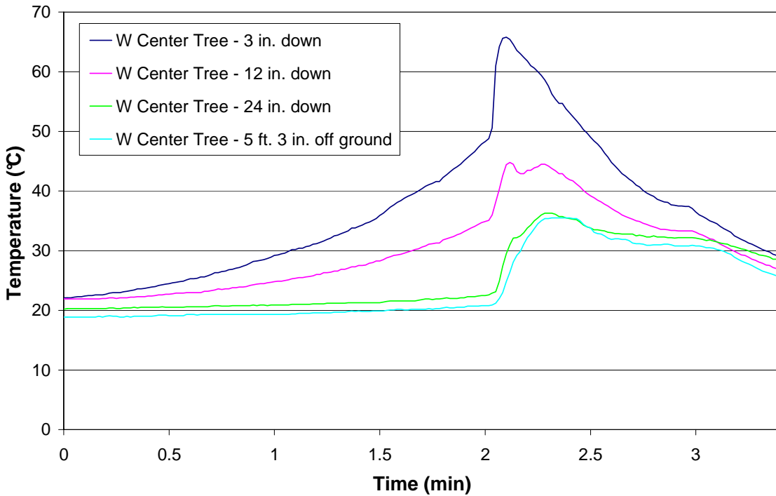
Figure 46 – Test 11 W Center Tree
