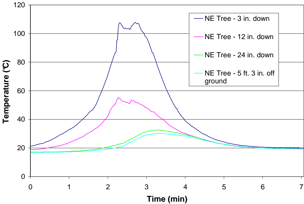
Figure 12 – Test 5 NE Tree
