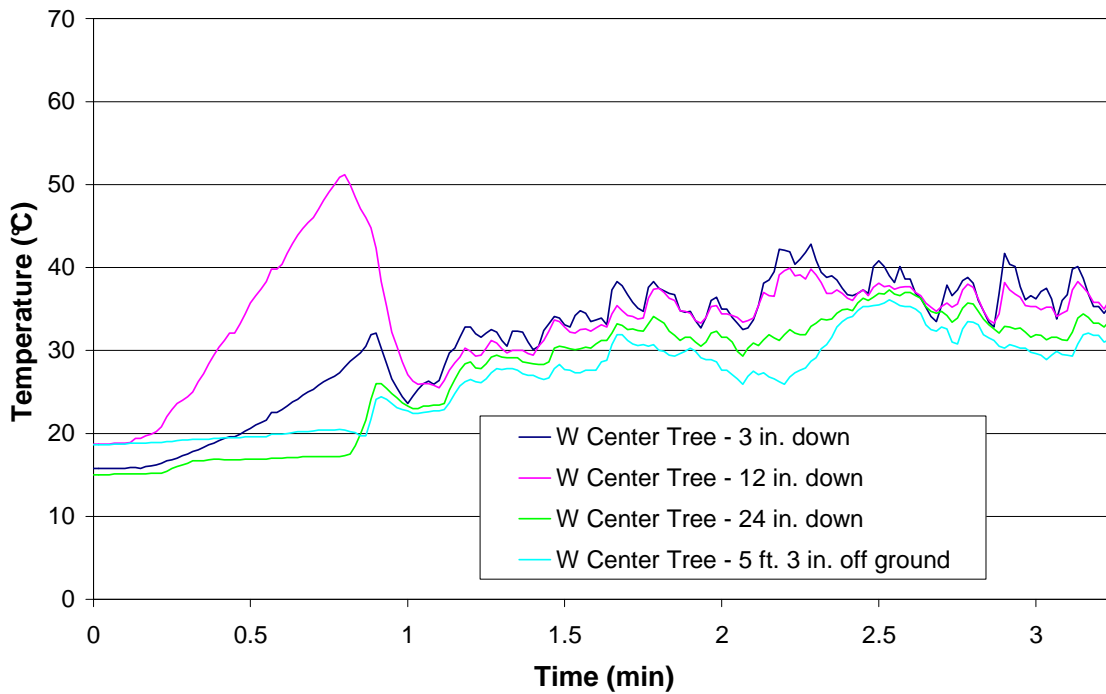
Figure 22 – Test 7 W Center Tree
