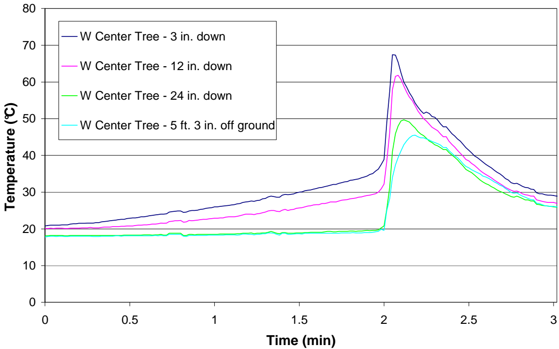
Figure 64 – Test 14 W Center Tree
