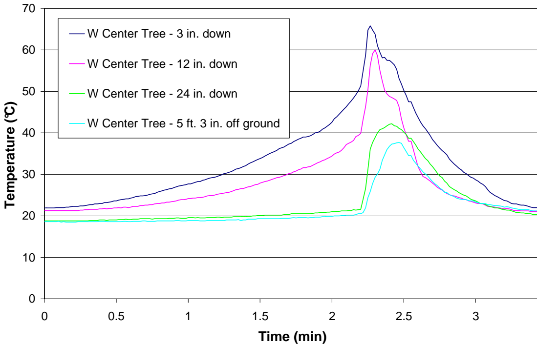
Figure 34 – Test 9 W Center Tree
