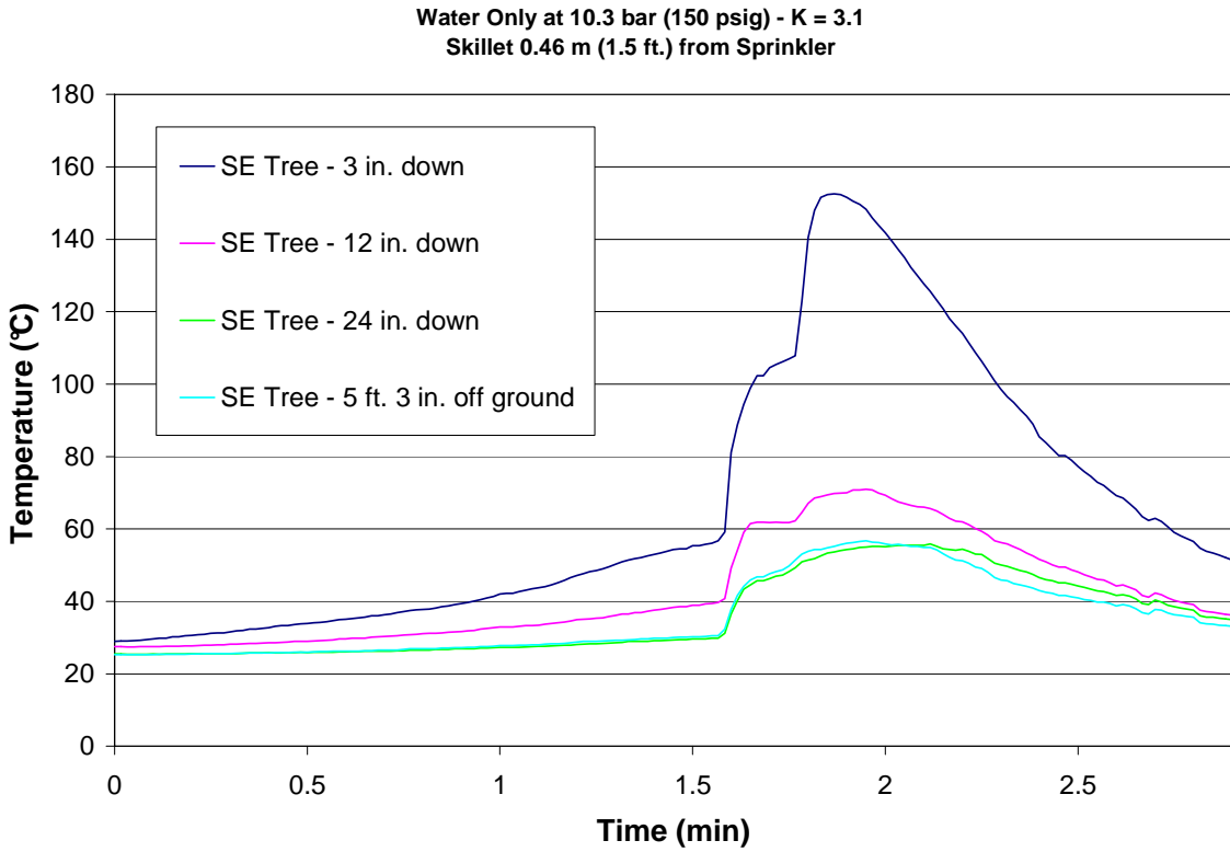
Figure 68 – Test 15 SE Tree
