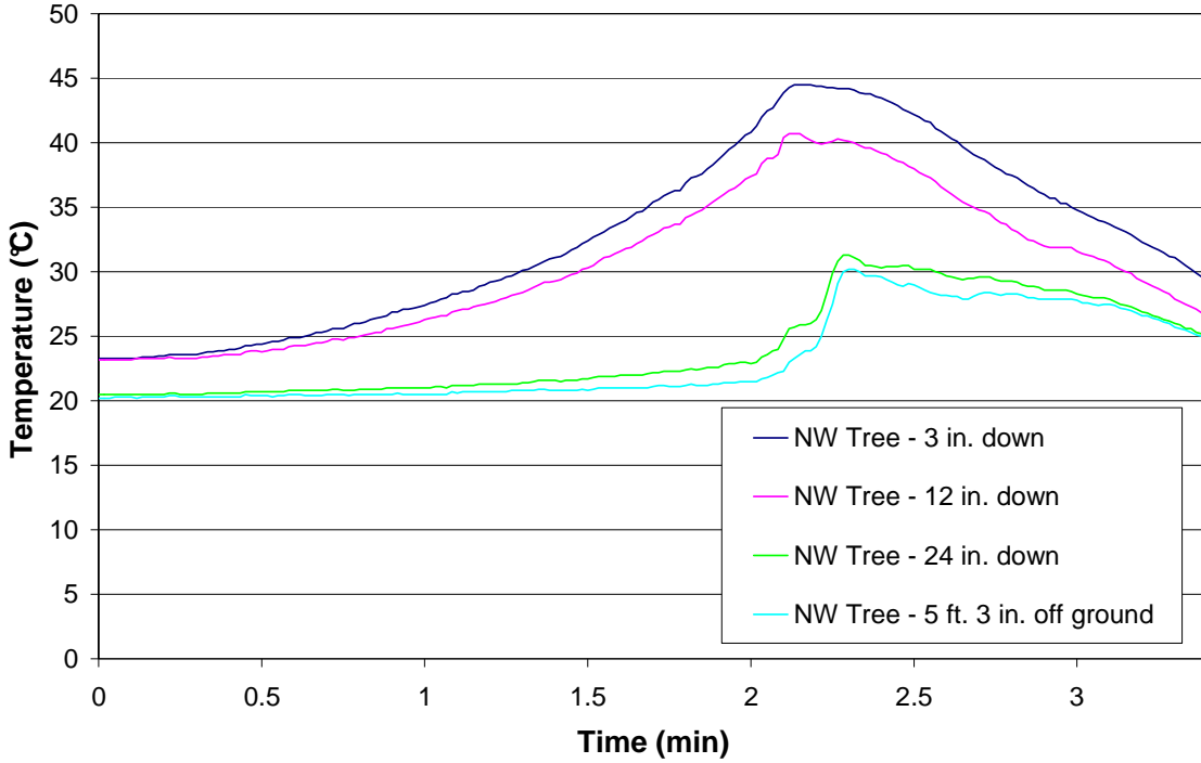
Figure 47 – Test 11 NW Tree
