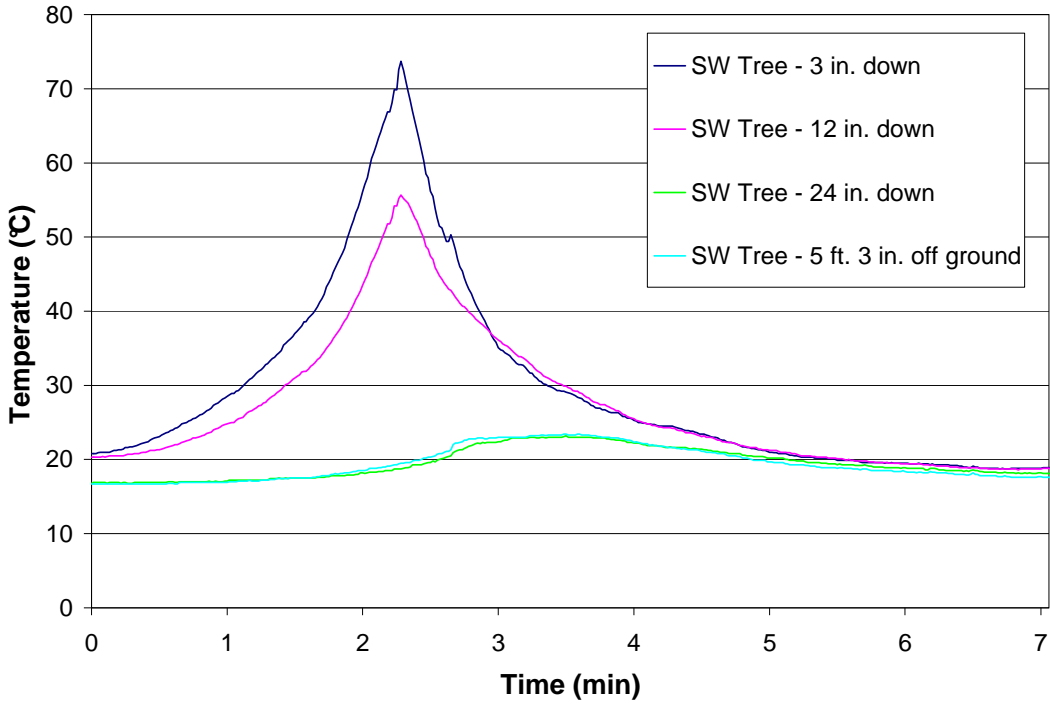
Figure 9 – Test 5 SW Tree
