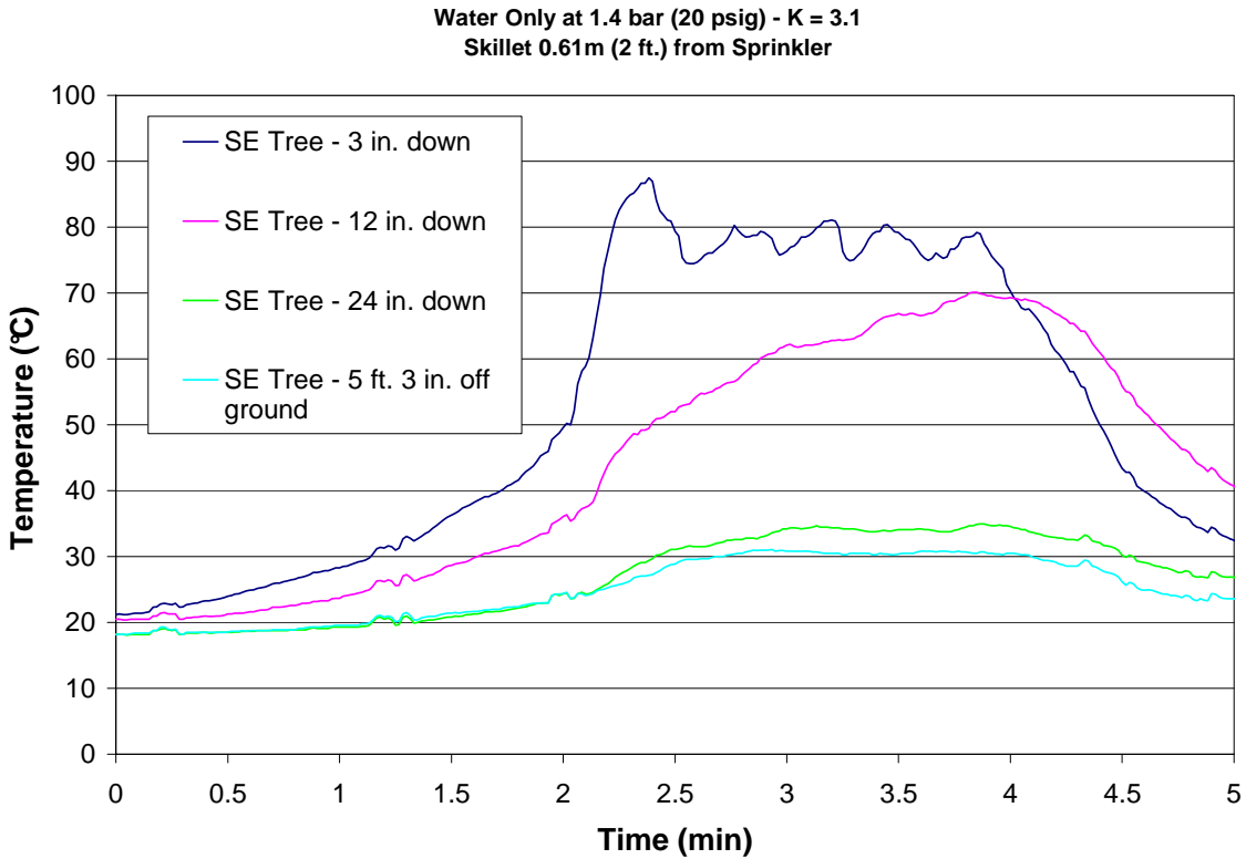
Figure 56 – Test 13 SE Tree
