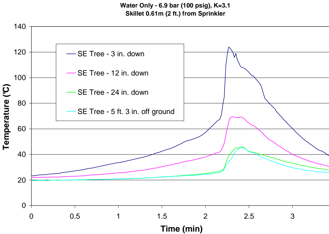
Figure 32 – Test 9 SE Tree
