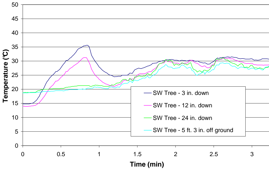
Figure 21 – Test 7 SW Tree
