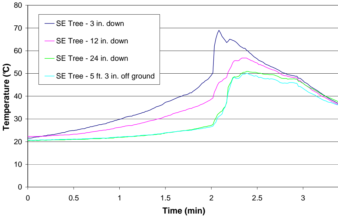
Figure 44 – Test 11 SE Tree
