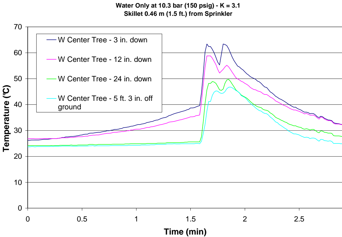
Figure 70 – Test 15 W Center Tree
