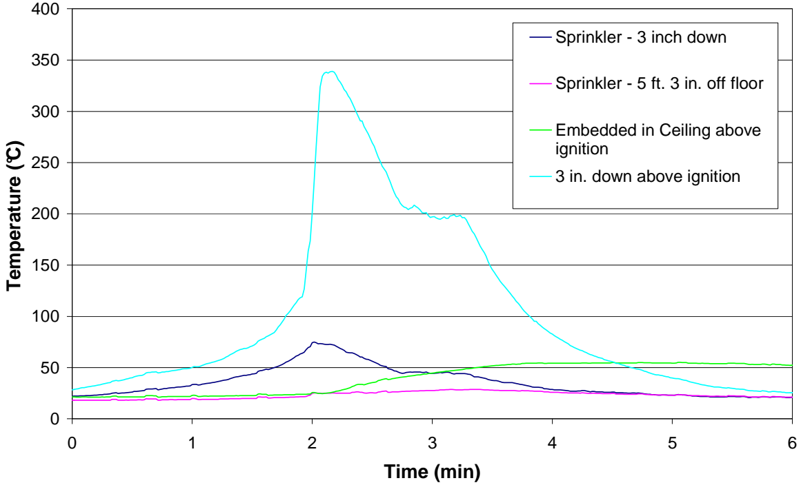
Figure 49 – Test 12 Sprinkler and Ignition Temperatures
