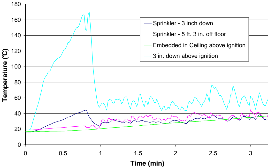
Figure 19 – Test 7 Sprinkler and Ignition Temperatures
