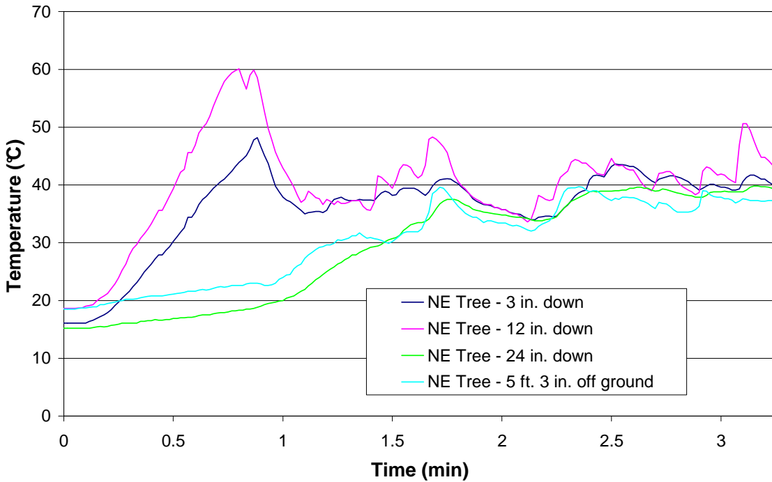
Figure 24 – Test 7 NE Tree
