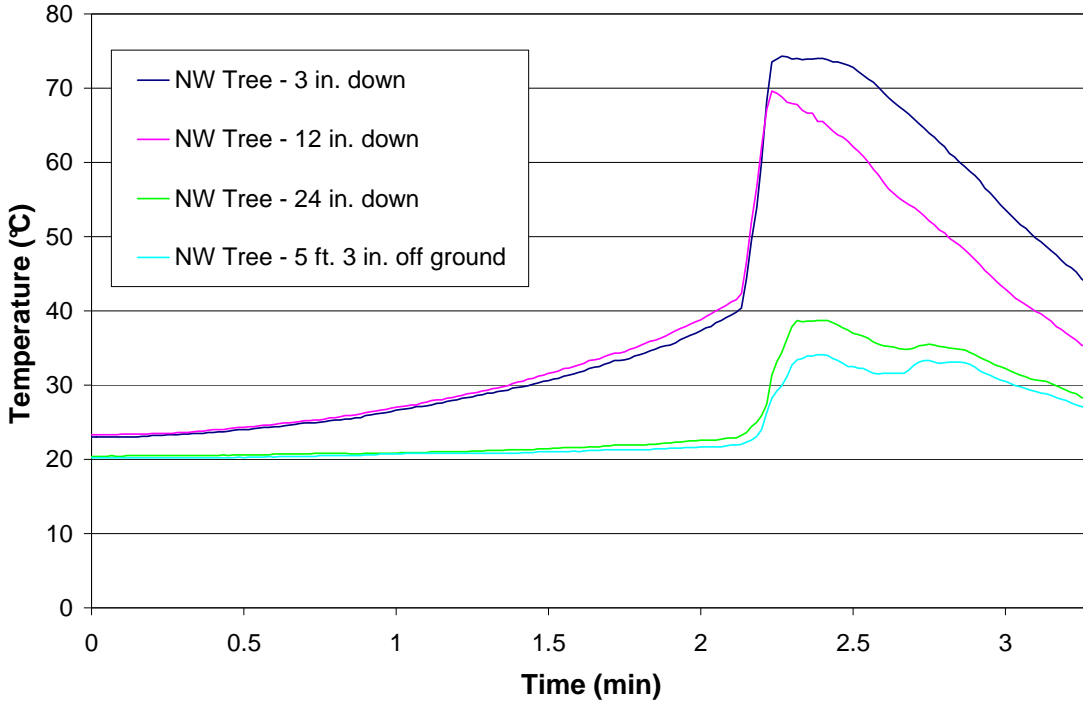
Figure 29 – Test 8 NW Tree
