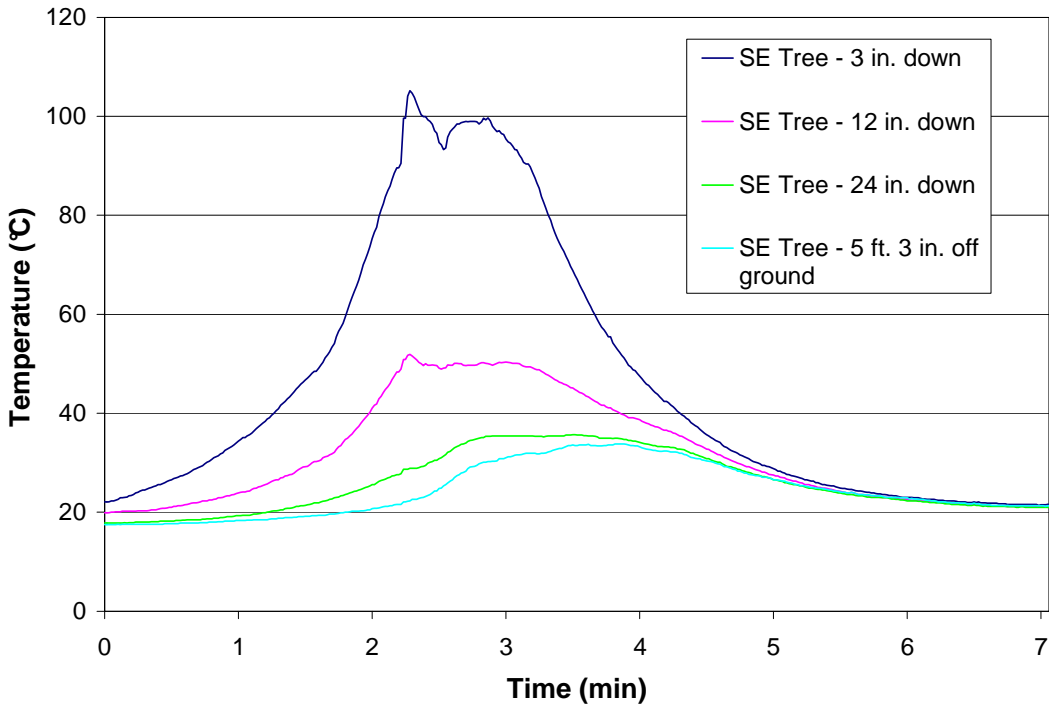
Figure 8 – Test 5 SE Tree
