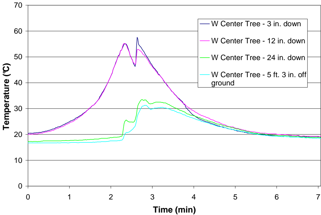
Figure 10 – Test 5 W Center Tree
