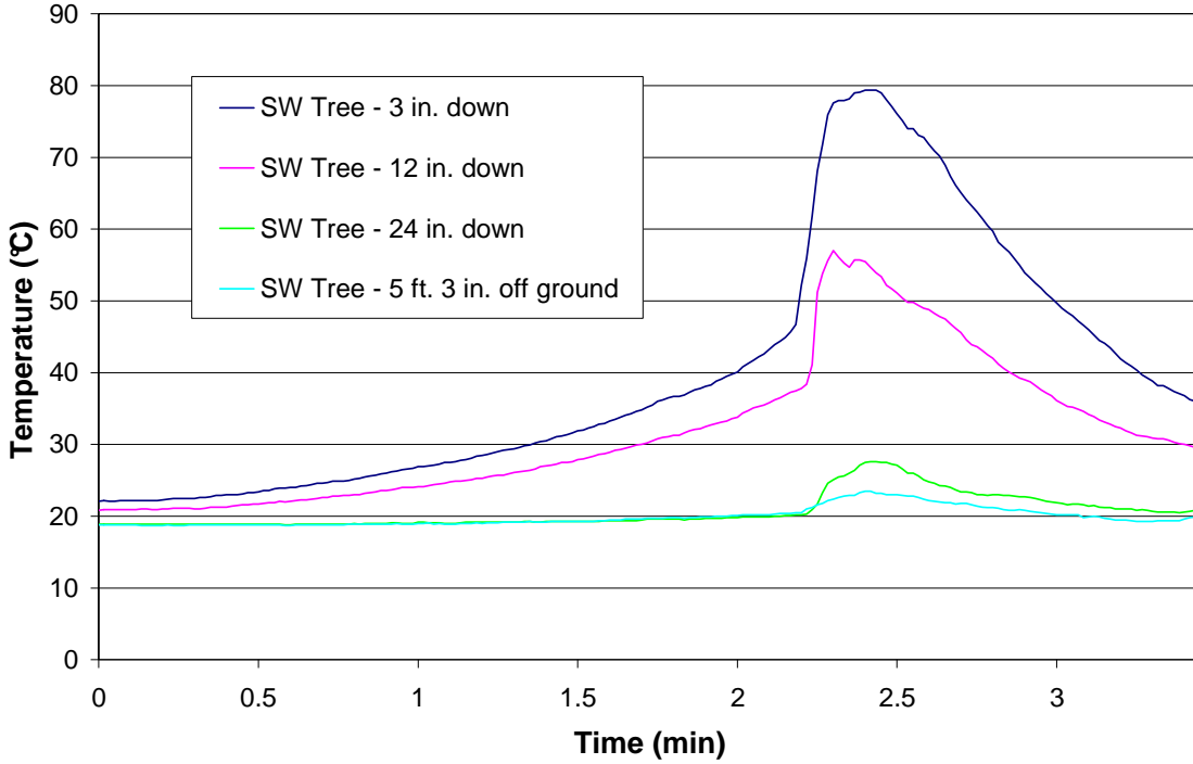
Figure 33 – Test 9 SW Tree
