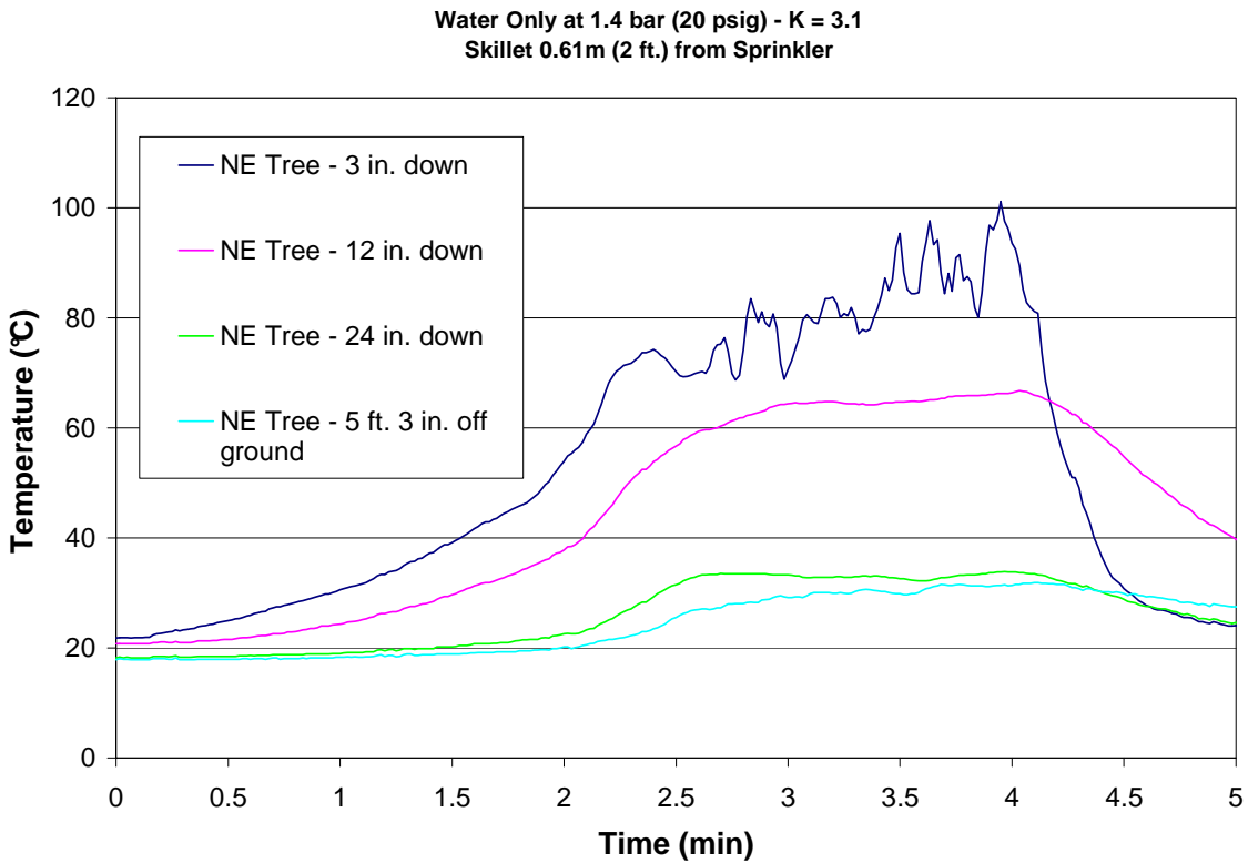
Figure 60 – Test 13 NE Tree
