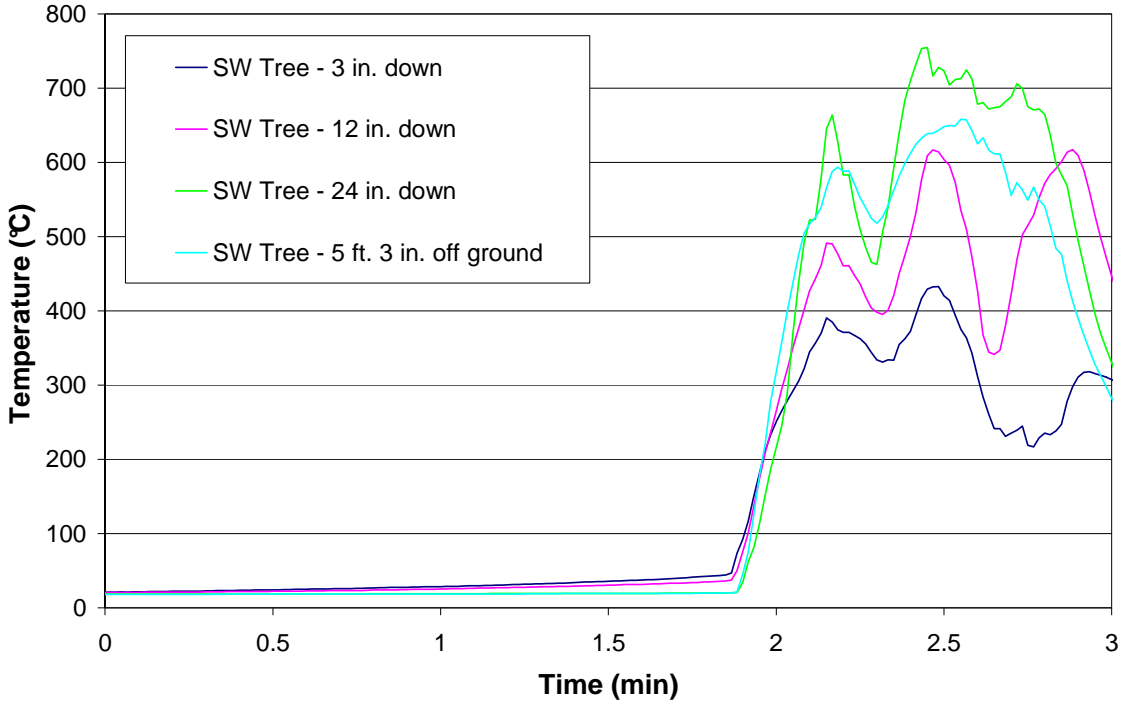
Figure 15 – Test 6 SW Tree
