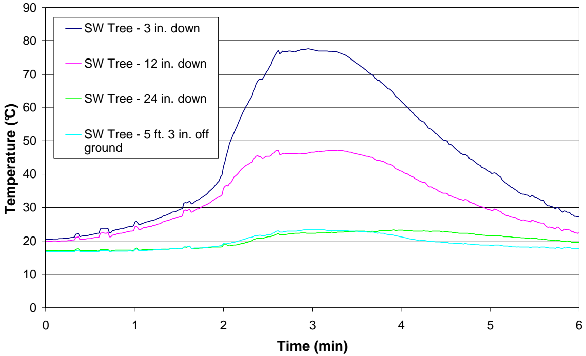
Figure 51 – Test 12 SW Tree
