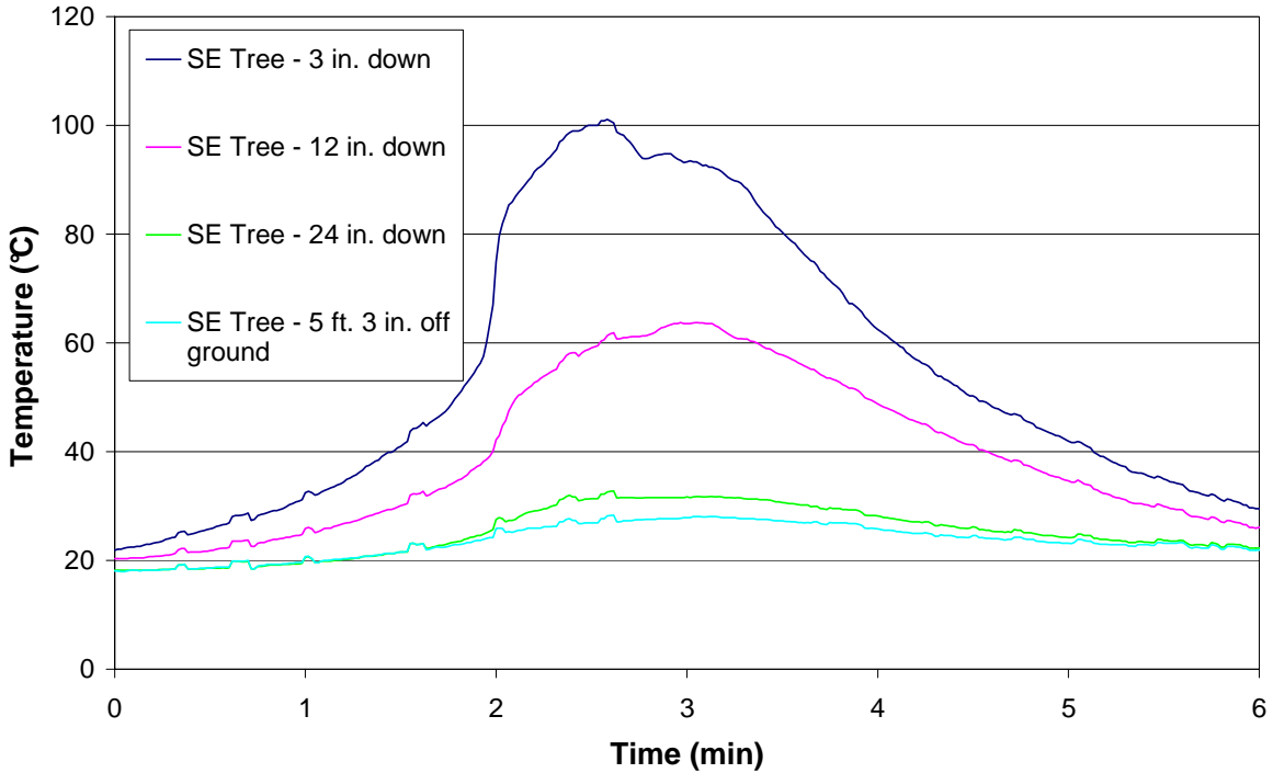
Figure 50 – Test 12 SE Tree
