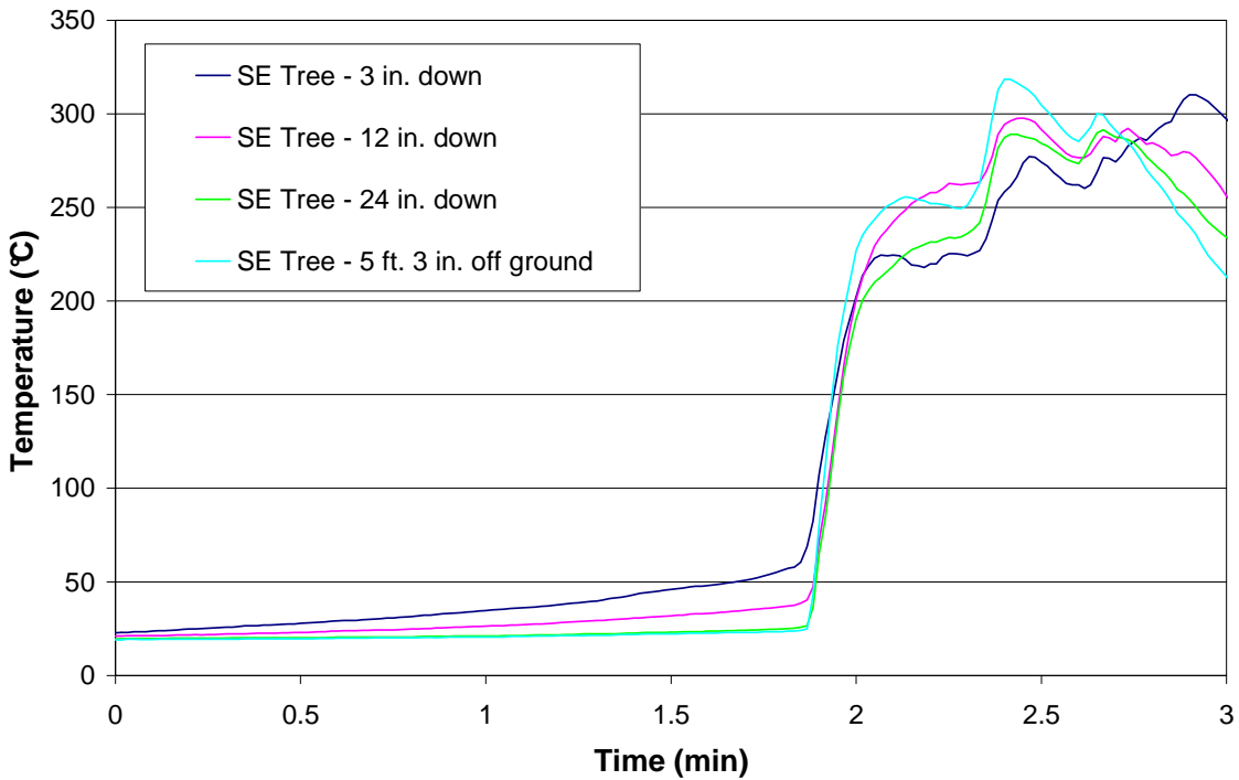
Figure 14 – Test 6 SE Tree
