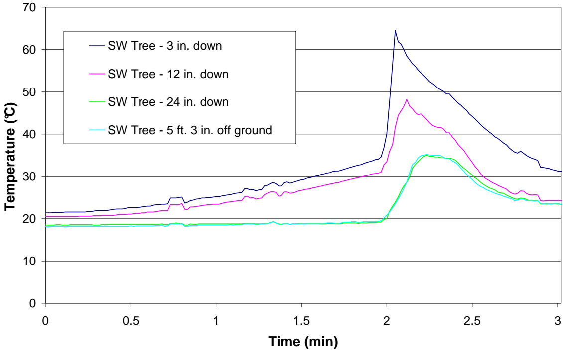
Figure 63 – Test 14 SW Tree
