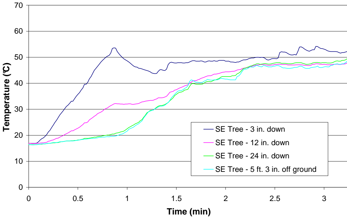
Figure 20 – Test 7 SE Tree
