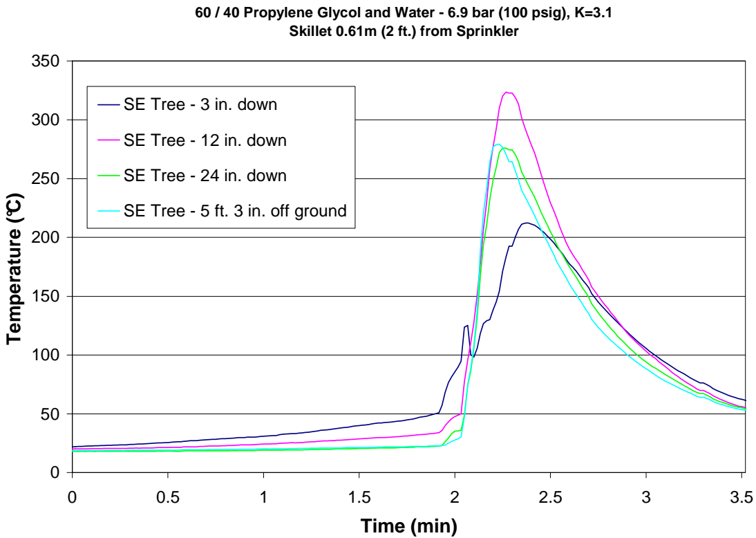
Figure 38 – Test 10 SE Tree
