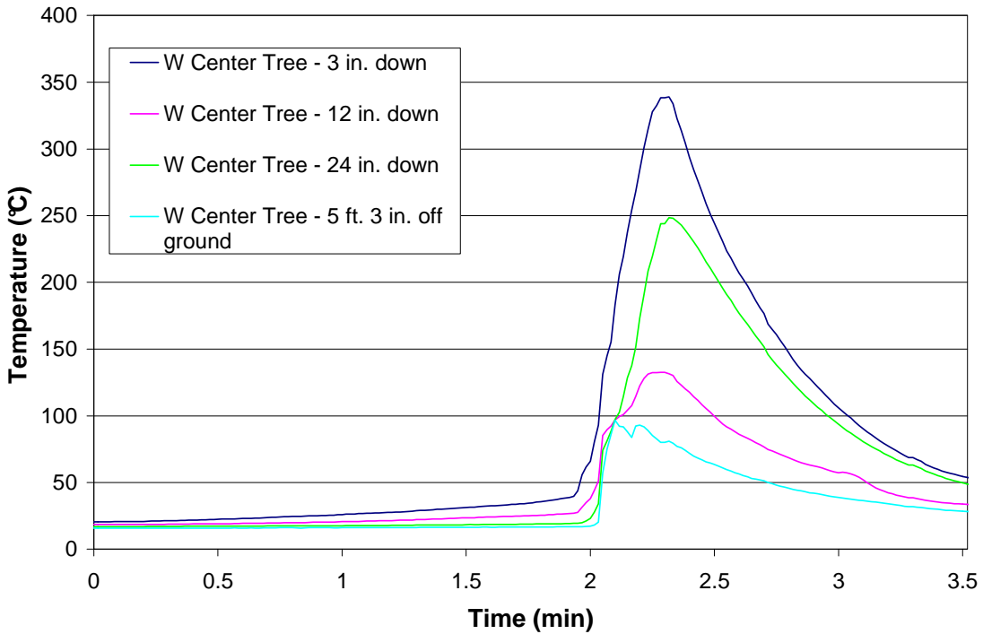
Figure 40 – Test 10 W Center Tree
