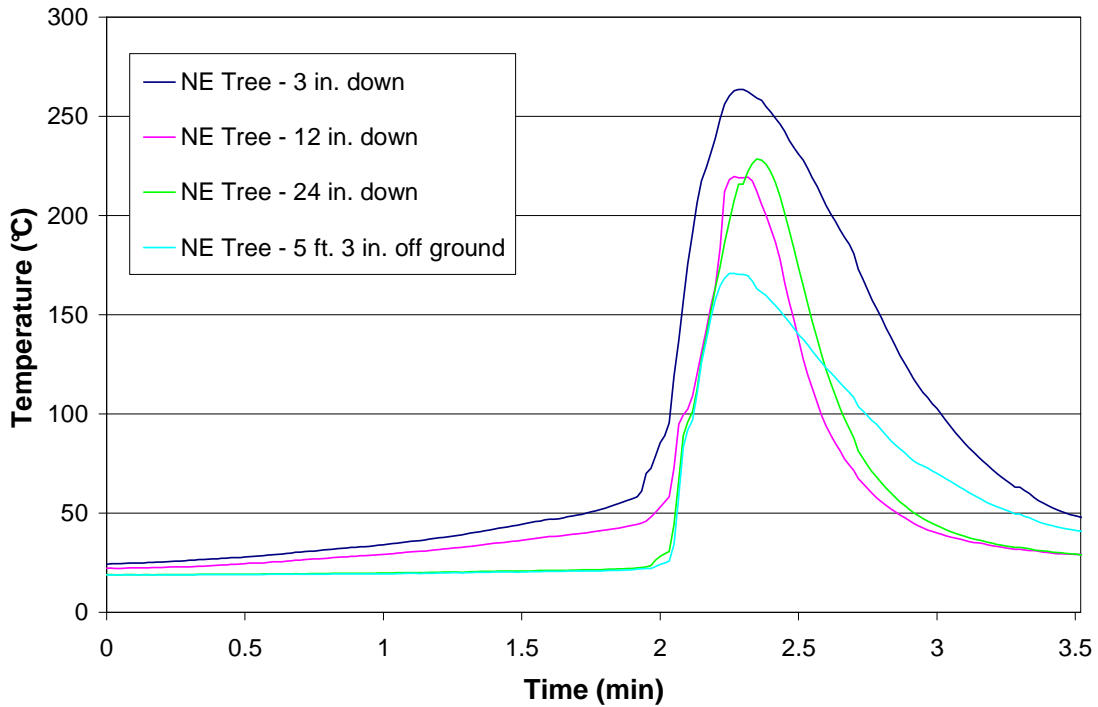
Figure 42 – Test 10 NE Tree
