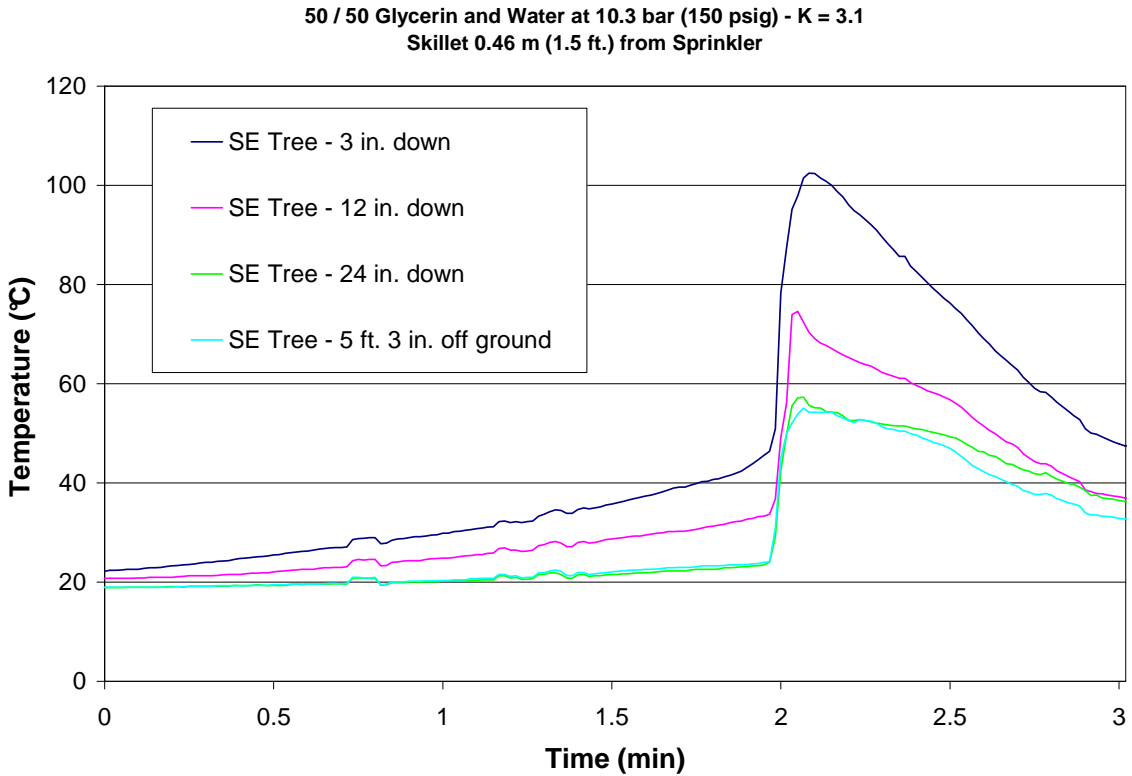
Figure 62 – Test 14 SE Tree
