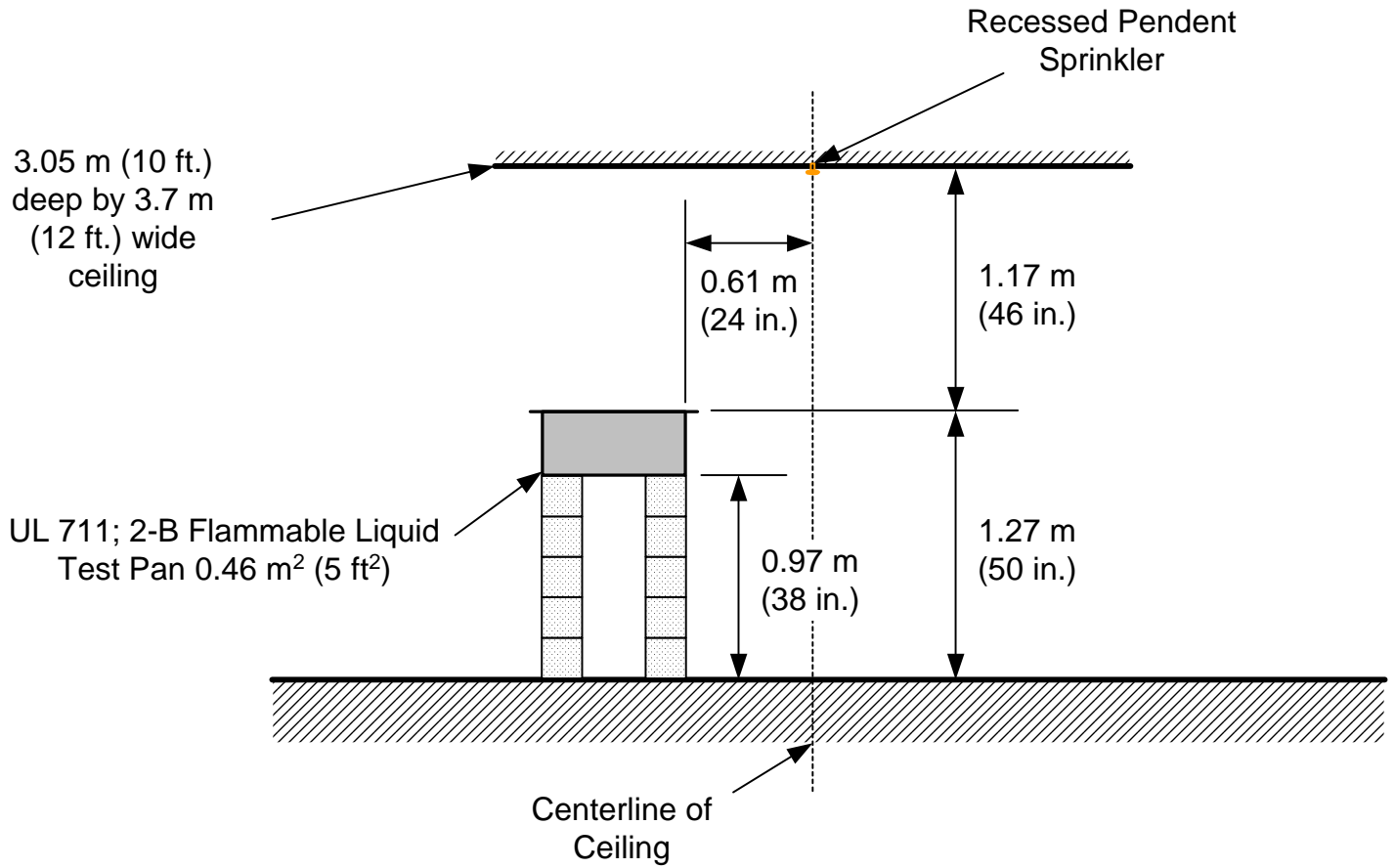
Figure 1 – Open Area Elevation View (Tests 1 – 4, 16 and 17)
