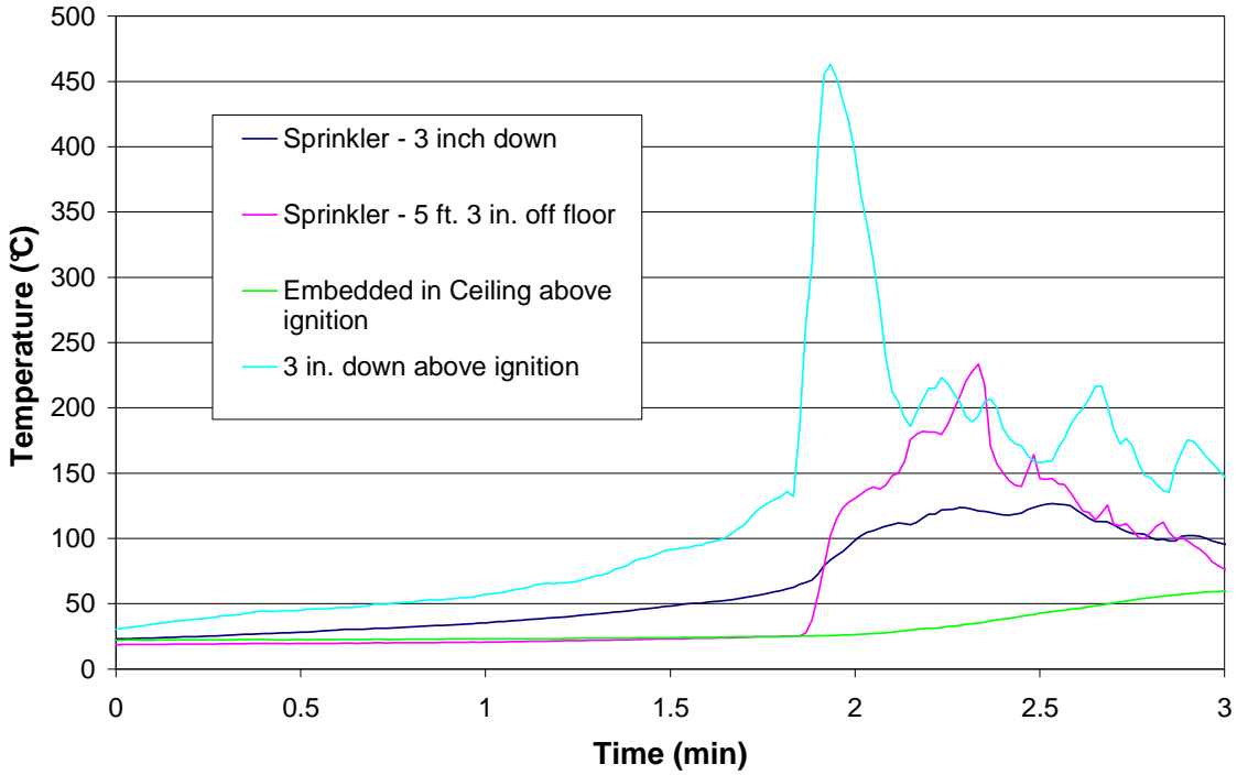
Figure 13 – Test 6 Sprinkler and Ignition Temperatures
