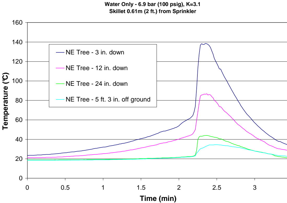
Figure 36 – Test 9 NE Tree
