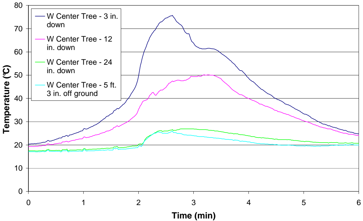
Figure 52 – Test 12 W Center Tree
