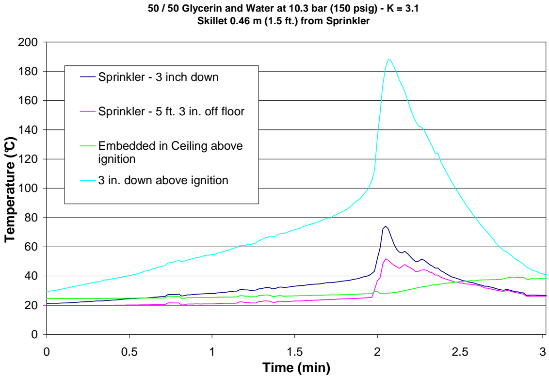
Figure 61 – Test 14 Sprinkler and Ignition Temperatures
