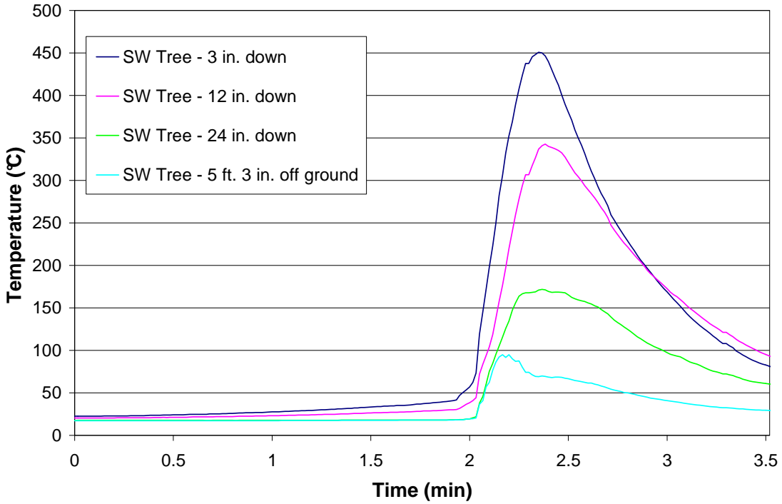
Figure 39 – Test 10 SW Tree
