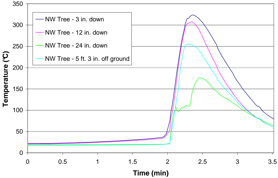
Figure 41 – Test 10 NW Tree
