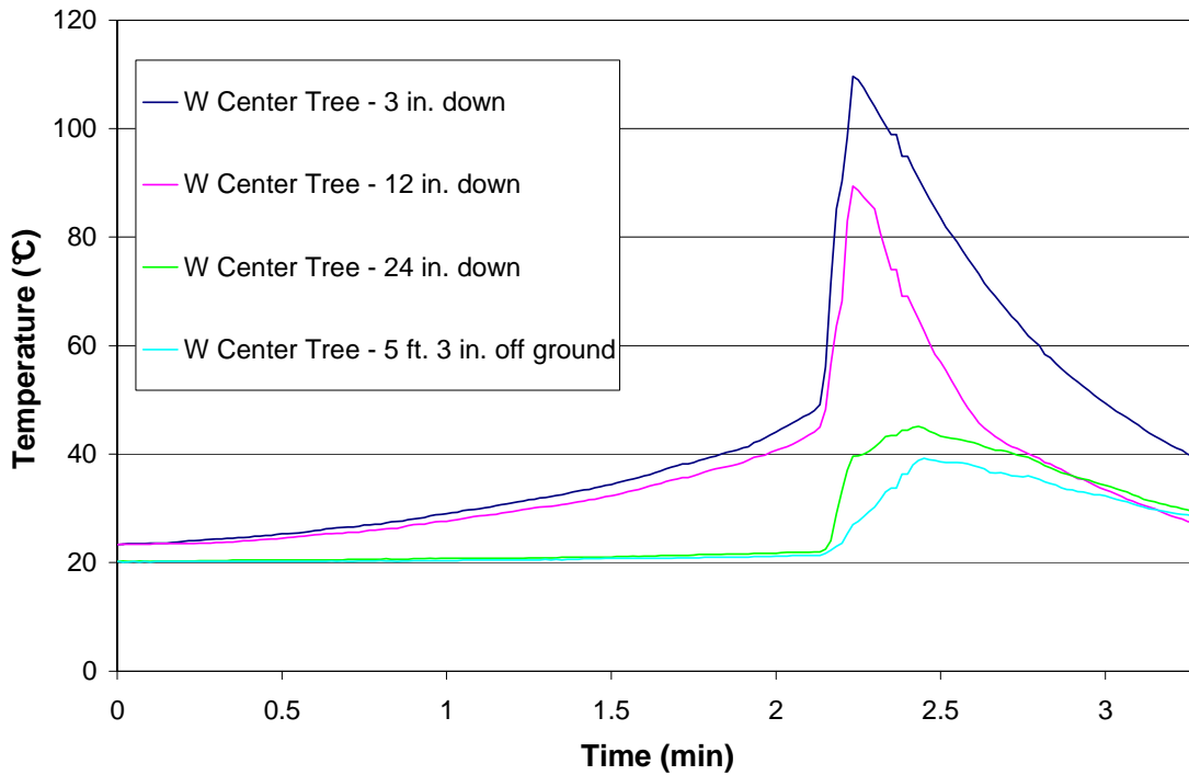
Figure 28 – Test 8 W Center Tree
