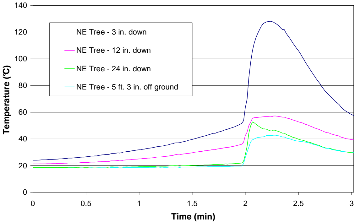
Figure 66 – Test 14 NE Tree
