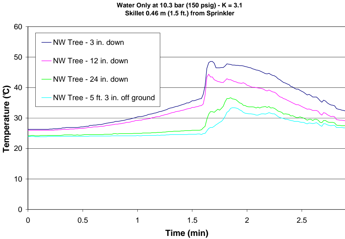
Figure 71 – Test 15 NW Tree
