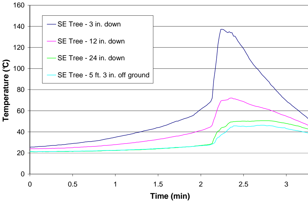
Figure 26 – Test 8 SE Tree
