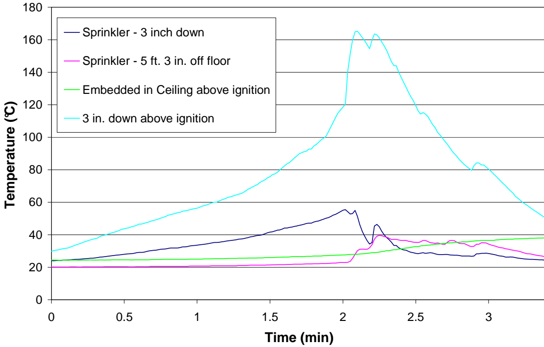
Figure 43 – Test 11 Sprinkler and Ignition Temperatures
