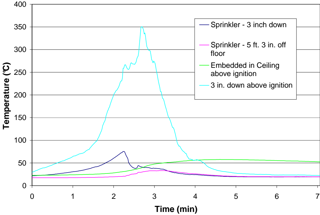
Figure 7 – Test 5 Sprinkler and Ignition Temperatures
