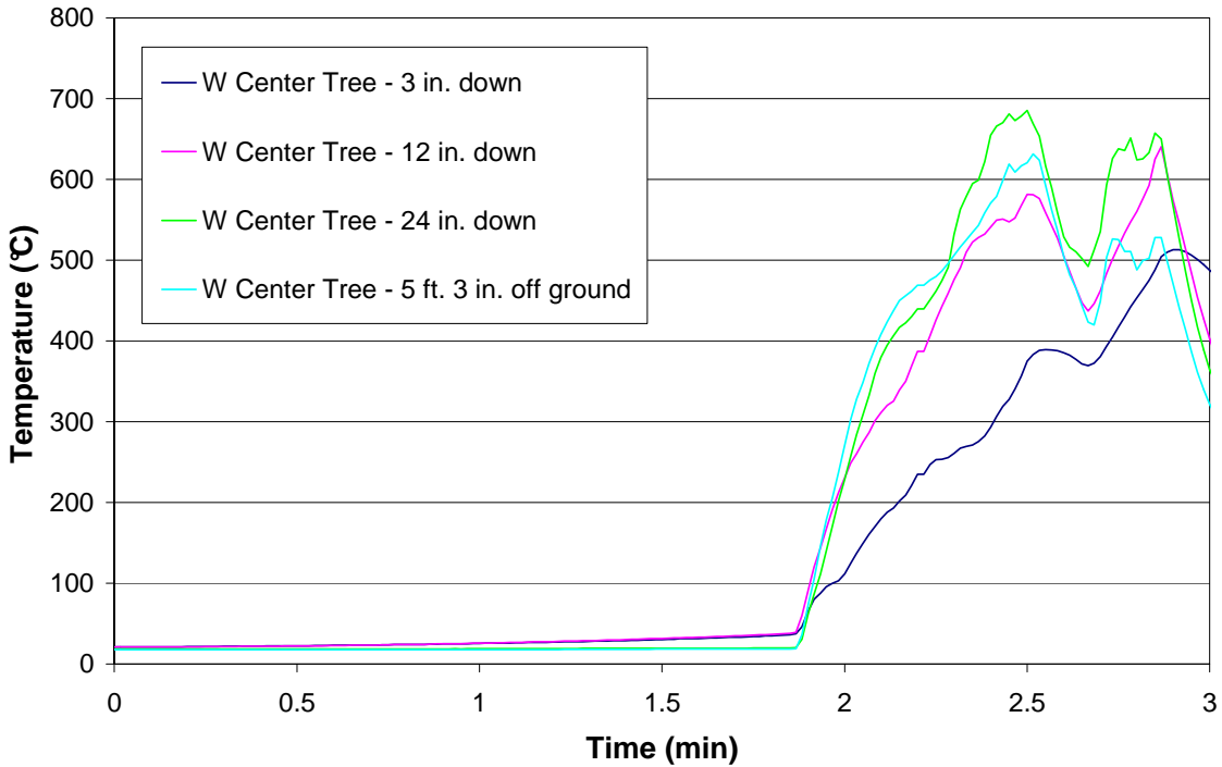
Figure 16 – Test 6 W Center Tree
