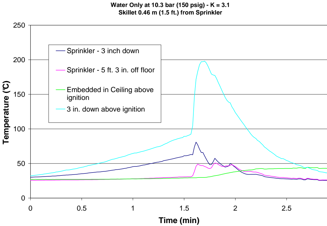
Figure 67 – Test 15 Sprinkler and Ignition Temperatures
