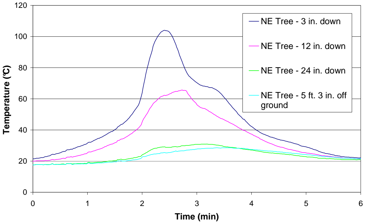
Figure 54 – Test 12 NE Tree
