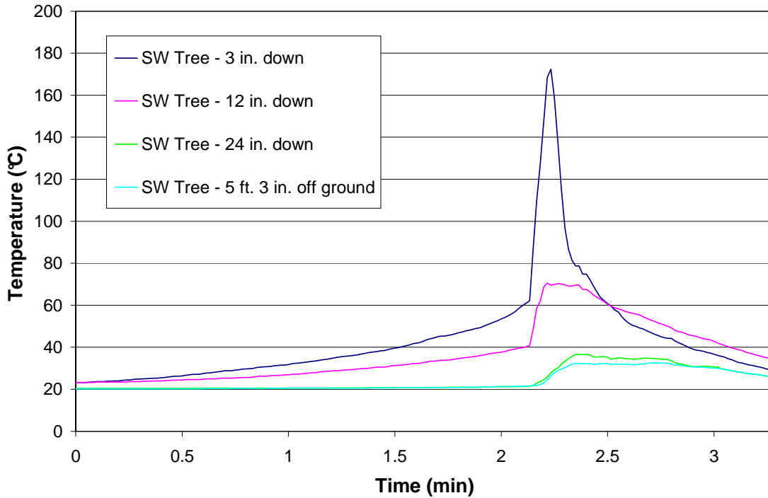
Figure 27 – Test 8 SW Tree
