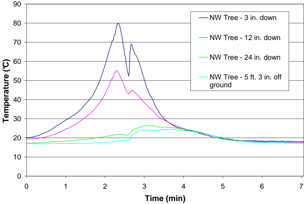
Figure 11 – Test 5 NW Tree
