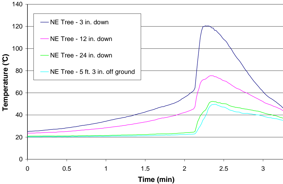
Figure 30 – Test 8 NE Tree
