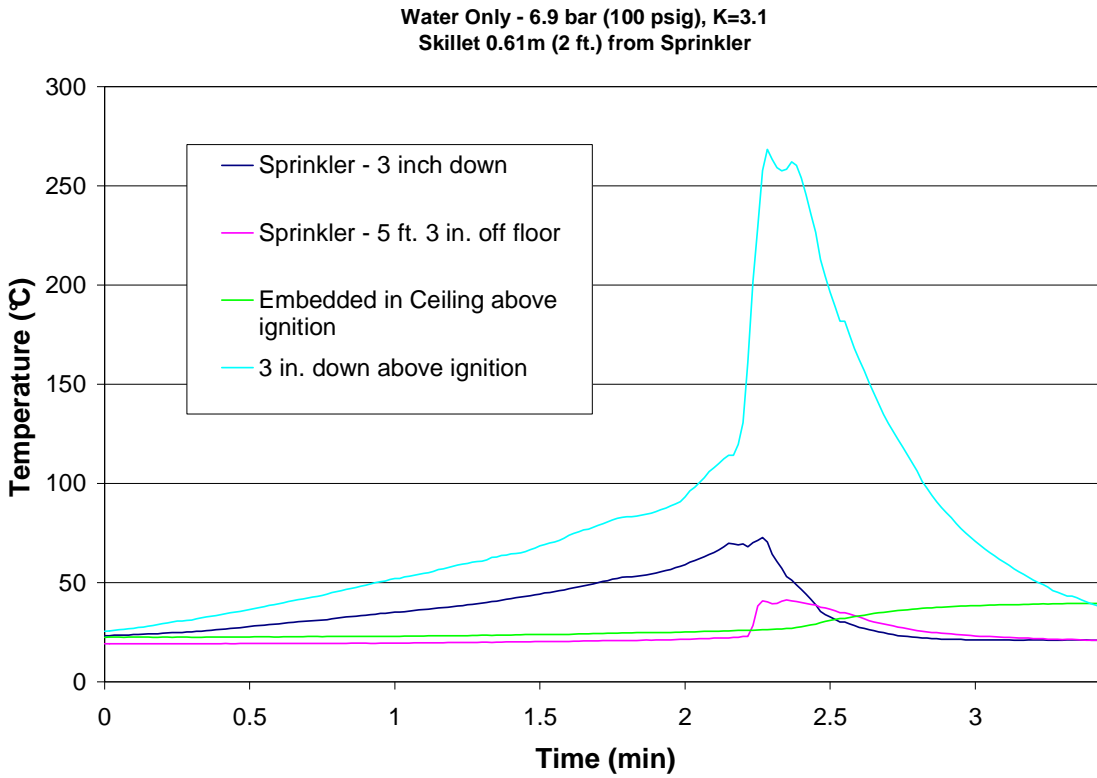
Figure 31 – Test 9 Sprinkler and Ignition Temperatures
