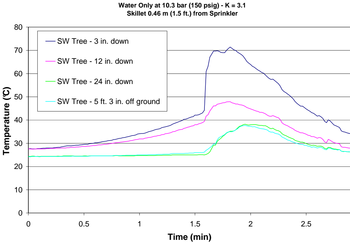
Figure 69 – Test 15 SW Tree
