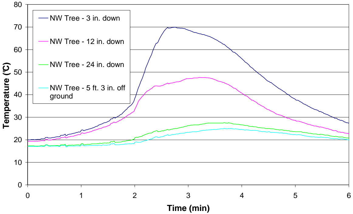
Figure 53 – Test 12 NW Tree
