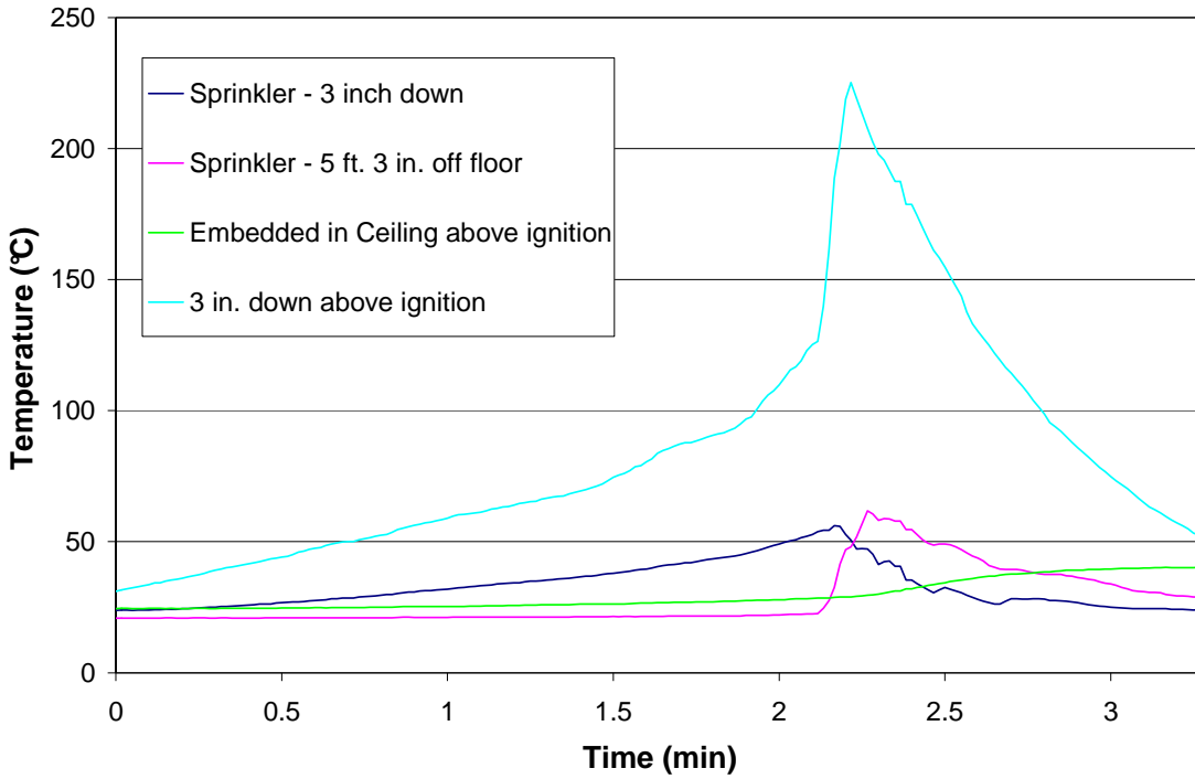
Figure 25 – Test 8 Sprinkler and Ignition Temperatures
