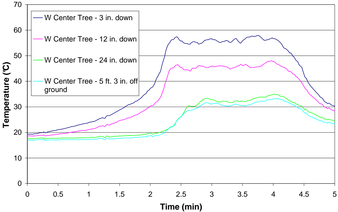
Figure 58 – Test 13 W Center Tree
