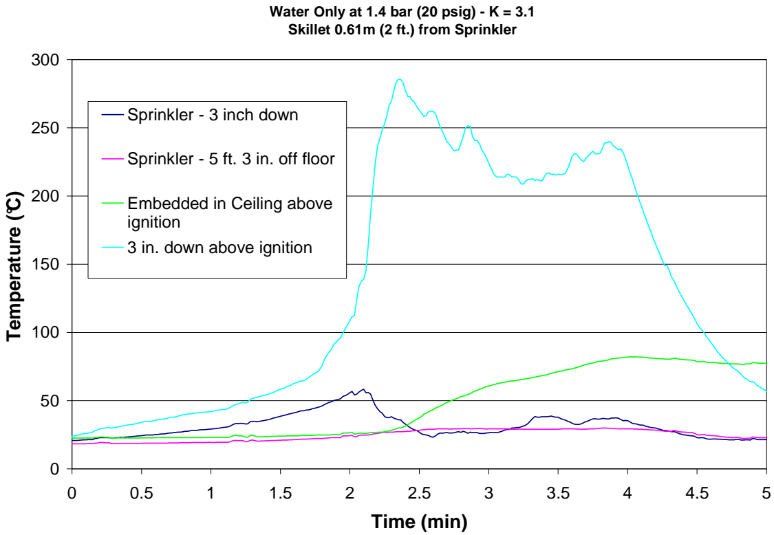
Figure 55 – Test 13 Sprinkler and Ignition Temperatures
