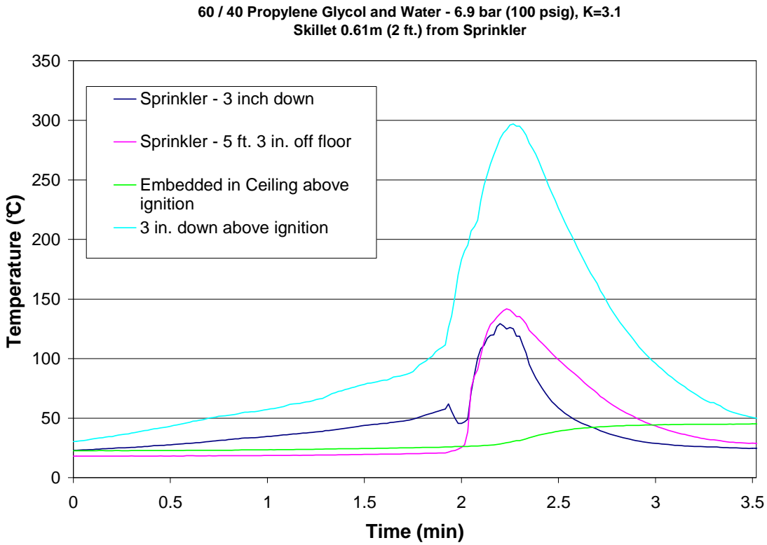
Figure 37 – Test 10 Sprinkler and Ignition Temperatures
