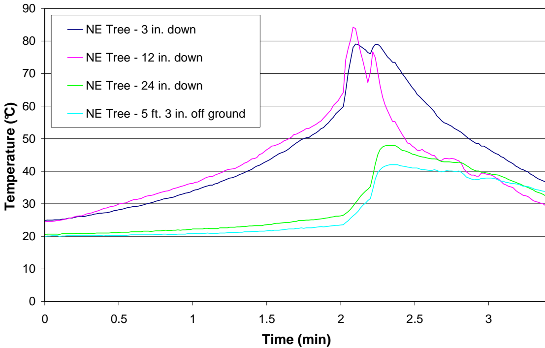
Figure 48 – Test 11 NE Tree
