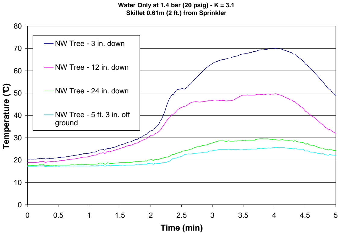
Figure 59 – Test 13 NW Tree
